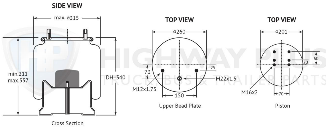
HP301-106A Airbag Assembly D30K
