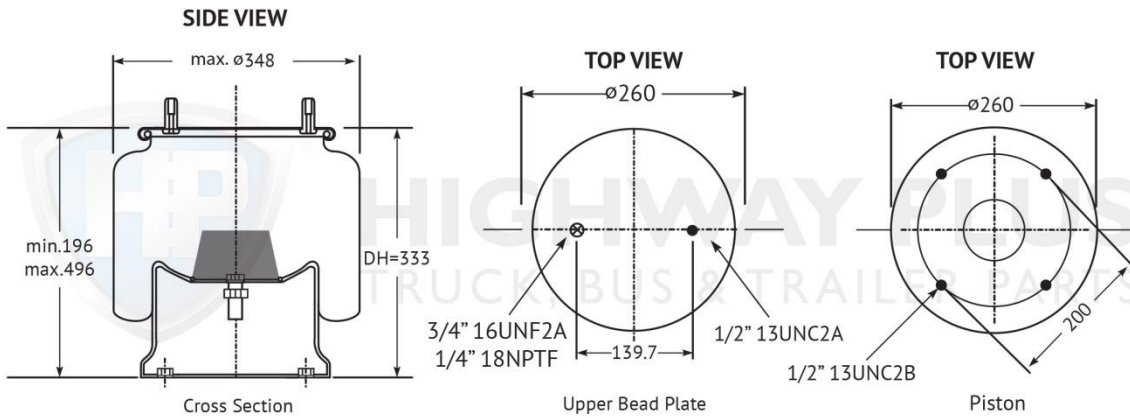
HP301-113 Airbag Neway
