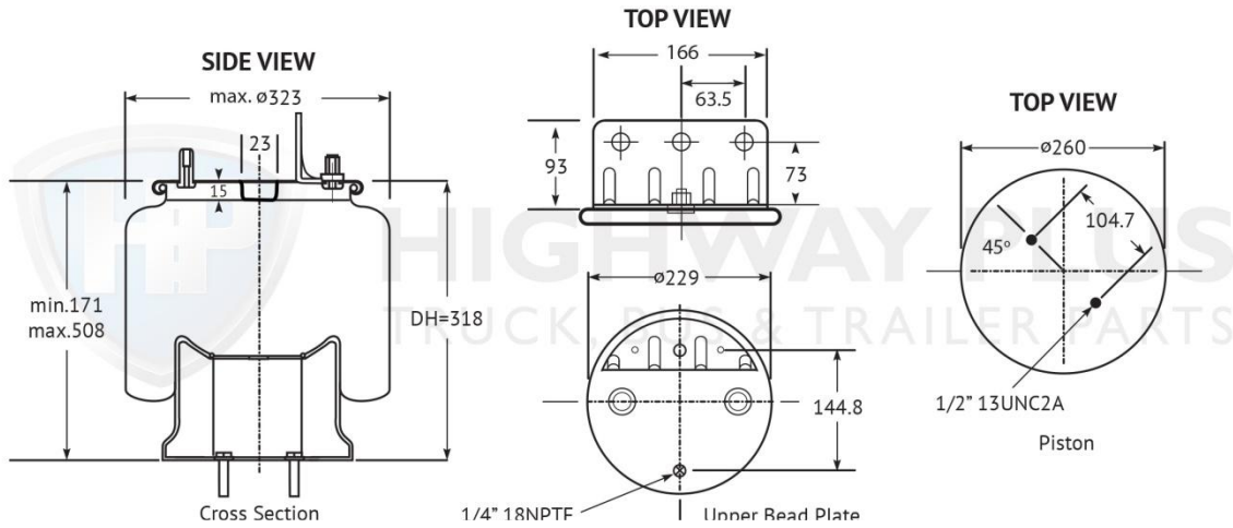
HP301-134 Airbag International
