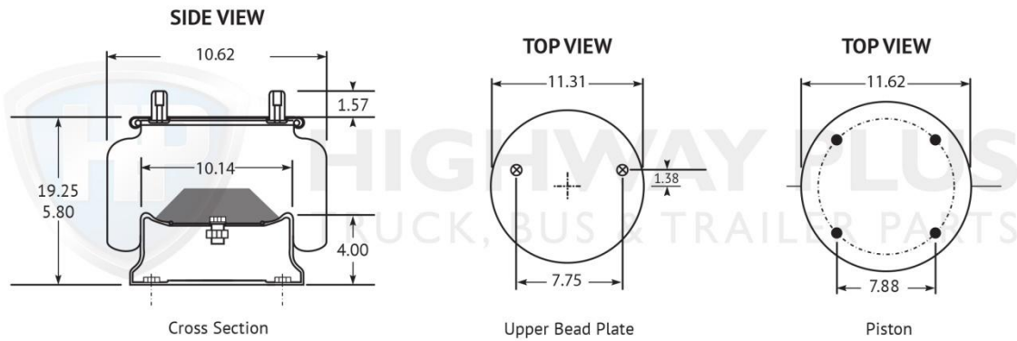
HP301-117 Airbag Hendrickson HT300
