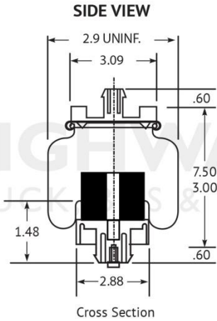
HP301-131 Airbag Cab Airspring - Freightliner
