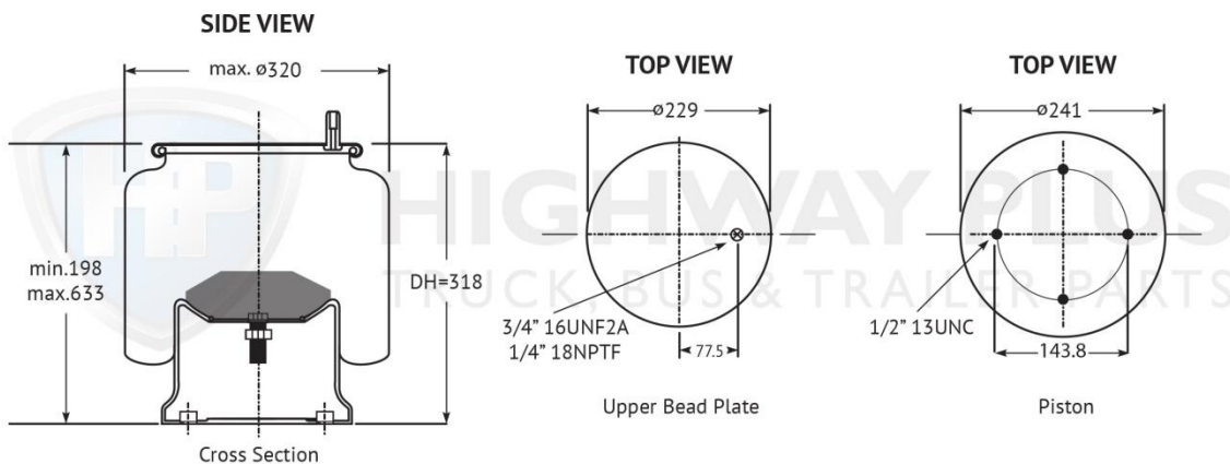
HP301-110 Airbag Hendrickson HT250U & UB
