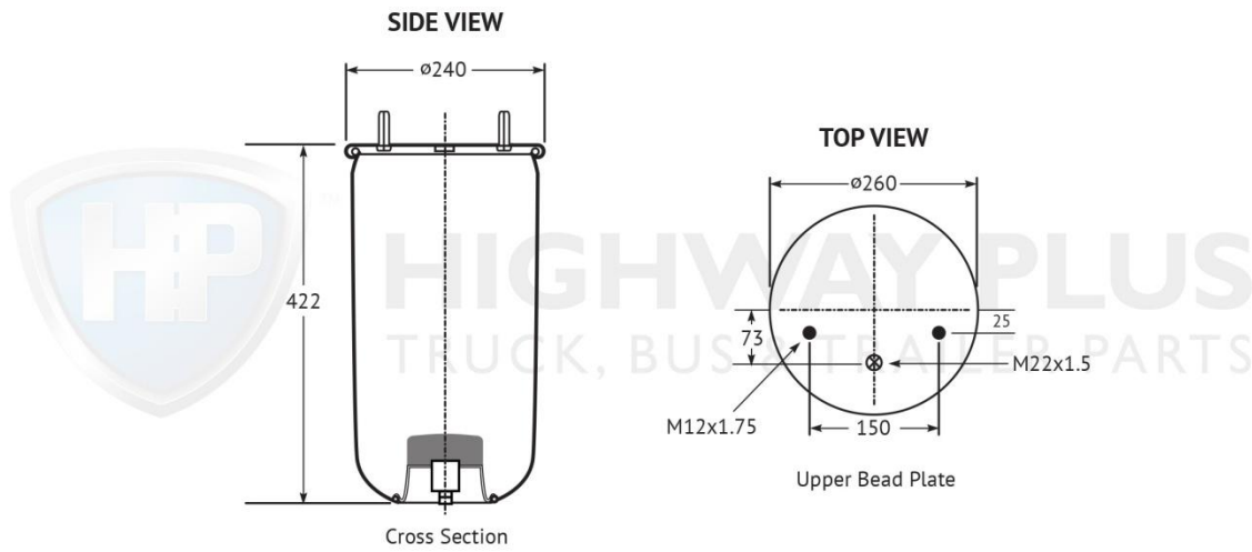
HP301-106 Airbag BPW D30K
