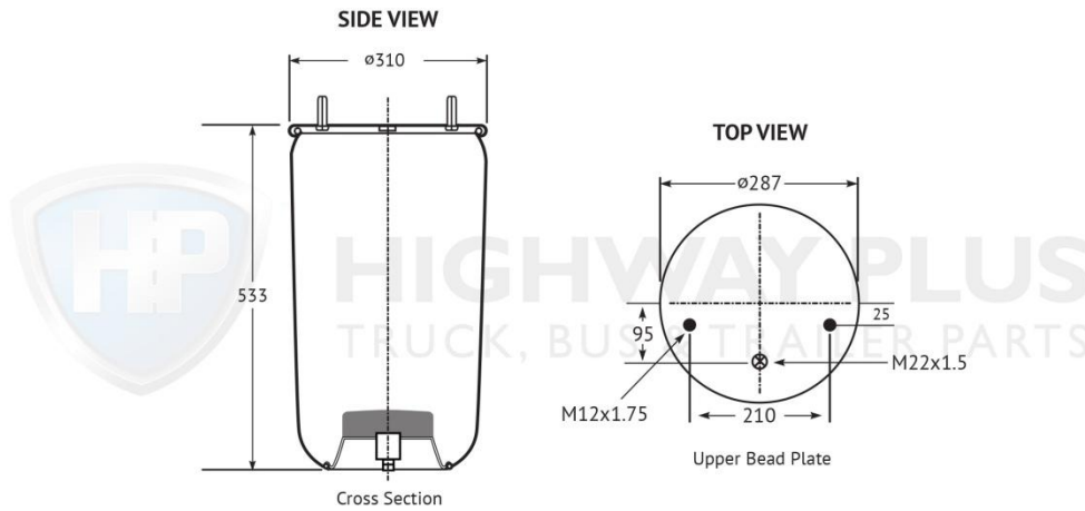
HP301-120 Airbag BPW Type 36
