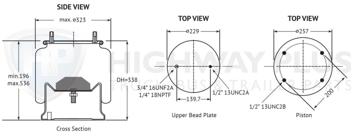
HP301-107 Airbag Assembly Neway SA38 SA44
