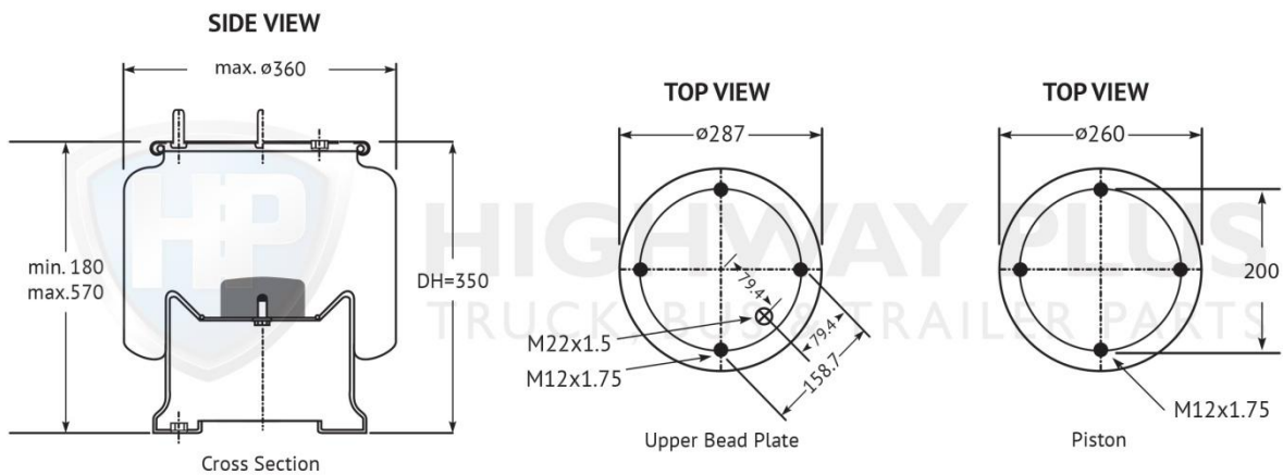
HP301-121 Airbag York ROR Weweller Holland
