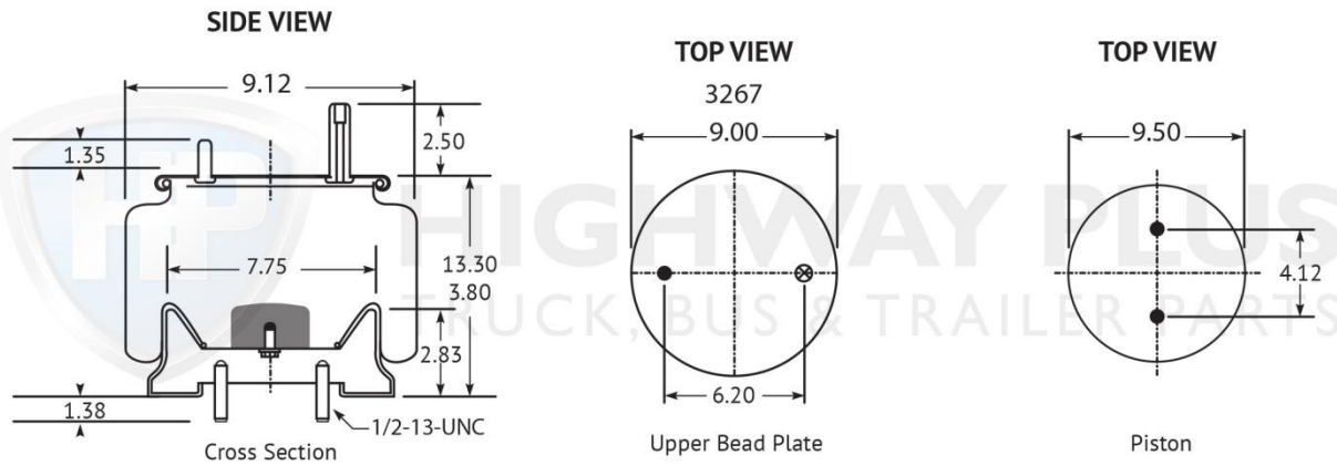
HP301-101 Airbag Kenworth Airslide 100
