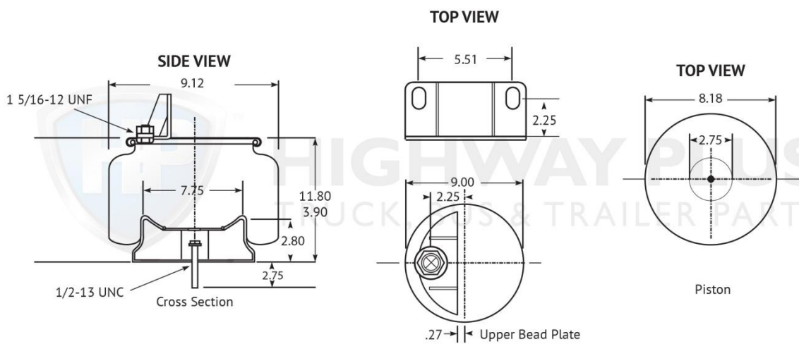
HP301-130 Airbag Late Airglide 200/460/690
