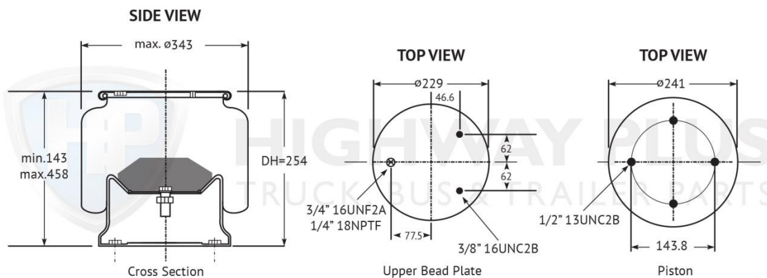
HP301-116 Airbag Hendrickson HT230
