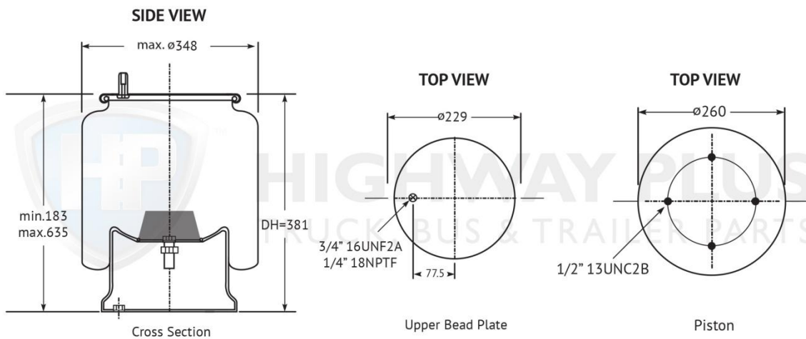
HP301-115 Airbag Hendrickson HT250 Us
