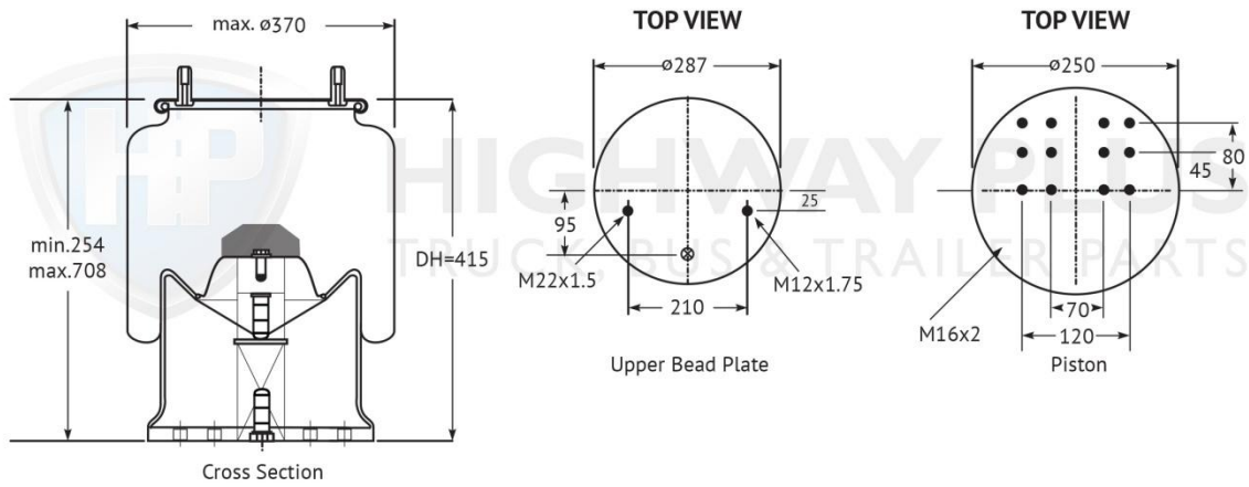
HP301-120A Airbag BPW Assembly Type 36
