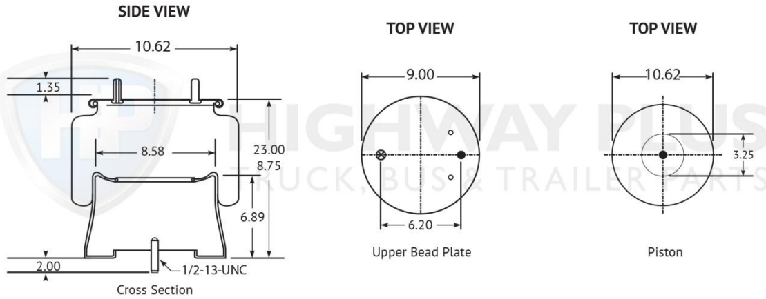
HP301-125 Airbag Freightliner
