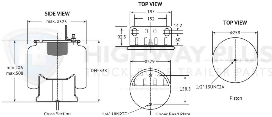
HP301-111 Airbag Hendrickson HAS
