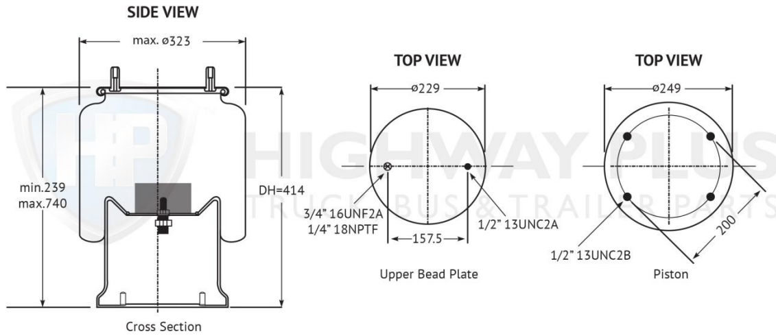
HP301-108 Airbag Hendrickson S14249
