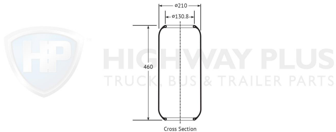
HP301-127 Airbag Volvo Mercedes BPW Van Hool
